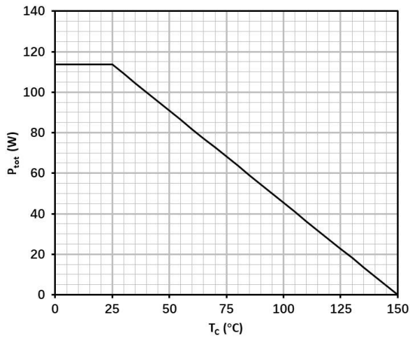
Figure 14 Power dissipation
